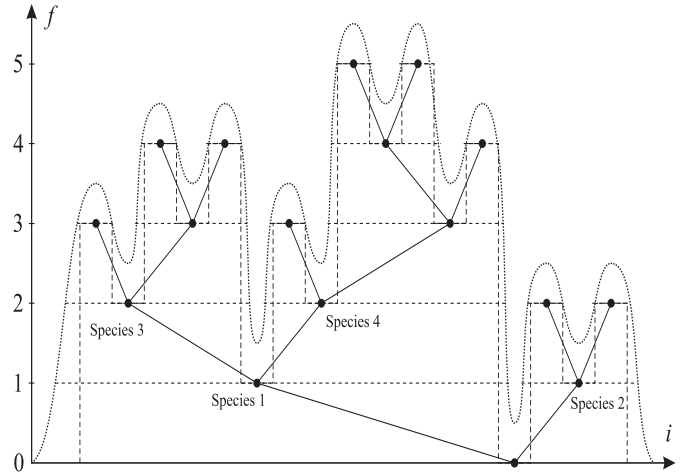
Figure 5: Generic fitness function with evolution tree. Individuals which are evolutionary neighbors are connected by a dashed line. They belong to the species indicated by a node on the dashed line. A species which can evolve from another is connected to it by a solid line. The smooth curve visualizes (somewhat misleading, since the fitness is discrete) the fitness function with many local maxima.
