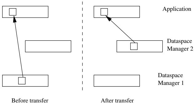
Figure 6. Modifying the semantics of a dataspace by moving the dataspace between managers.
